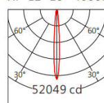
XP-E2 10° 4000K
