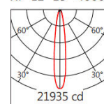
XP-E2 15° 4000K
